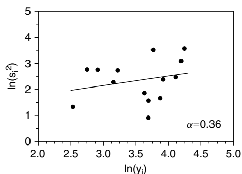
Figure 3.8. Log-log plot of changes in the variance ( s_i^2 ) of the i th sample mean as a function of the value of the i th sample mean ( y_i ). This plot is used in determination of the type of error present in the experimental data set for the establishment of a weighting scheme to be used in regression analysis of the data. The value of the slope of the line ( \alpha ) suggests a homogeneous, or constant, error in the experimental data.
