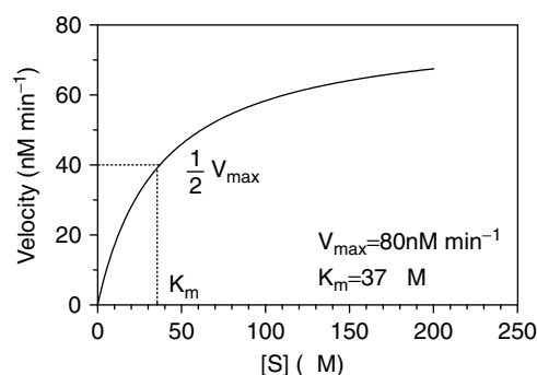
Figure 3.5. Initial velocity versus substrate concentration plot for an enzyme with V_{\max} = 80 \text{ nM min}^{-1} and K_m = 37 \mu\text{M} .
